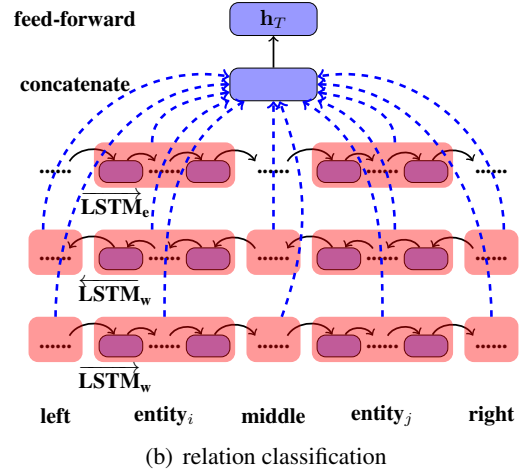
(b) relation classification
