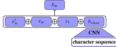
Figure 3: Word representations.
